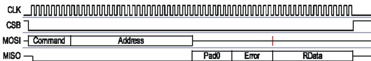
Figure 4: CSPI Register Read Cycle
