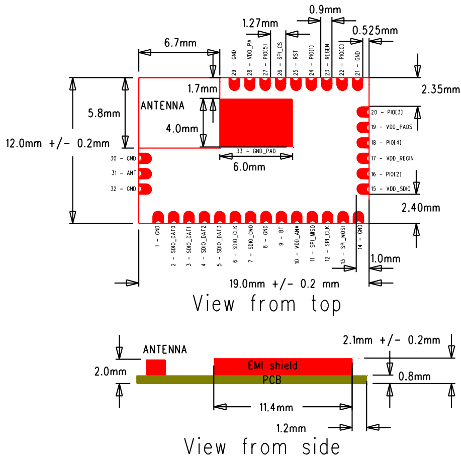
Figure 11: Physical dimensions
